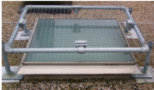
Figure 43 Covers can be fitted to existing roofs or included as part of the design (image courtesy of Safesite Limited)
